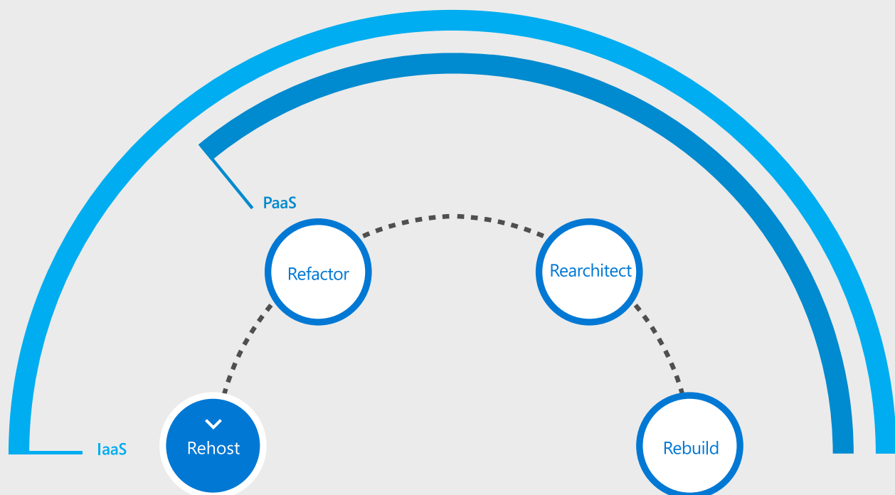
Figure 6. Migration strategies
