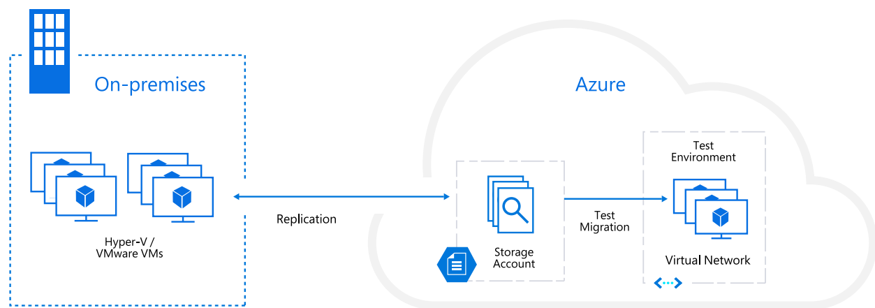
Figure 13. Test failover
